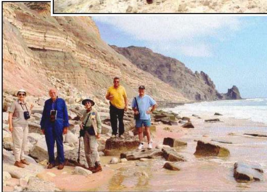
Sandstone and limestone cliffs between Lagos and Luz. Dark outcrop is basalt and explosion breccia volcanic neck and dolerite dyke.
